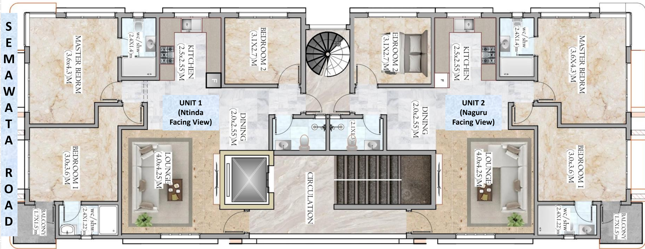
1 st , 2 nd , 4 th and 5 th Floor Layout
